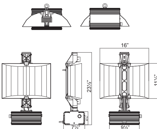
Main Dimension
